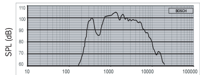
Frequency response
